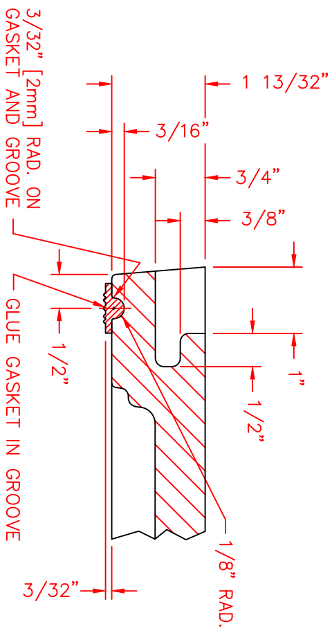
T-SEAL / CONCEALED PICK DETAIL HALF SCALE (GASKET NO. 02797)
