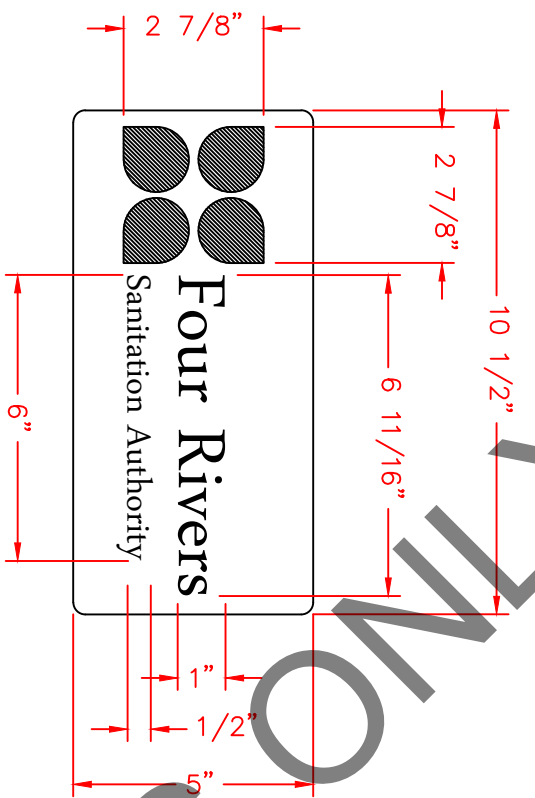
LOGO DETAIL SCALE = 1/4
