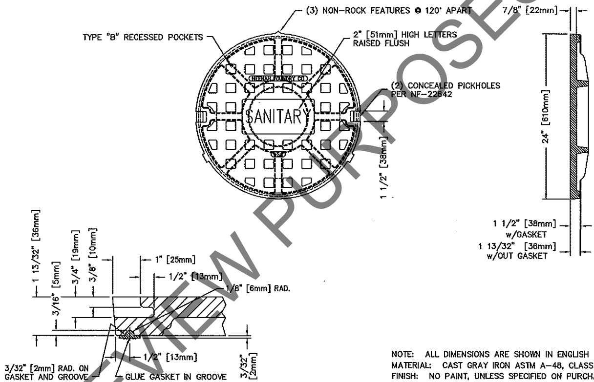
T-SEAL / CONCEALED PICK DETAIL HALF SCALE (GASKET NO. 02797)
